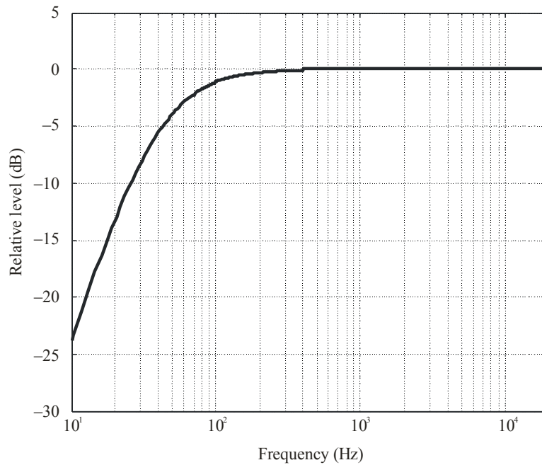
FIGURE 4 RLB weighting curve
