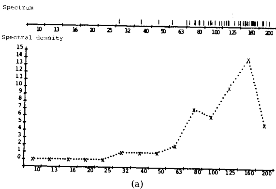
Fig. 12. Calculation of resonance modes: (a) 1.6:3:4; (b) 2:3:5.
