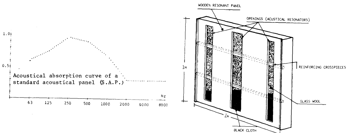
Fig. 13. Internal construction of a standard acoustical panel.
