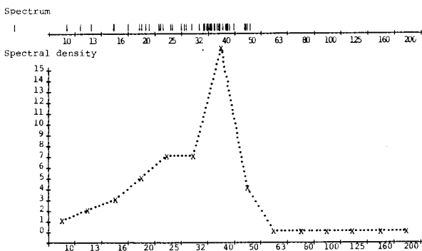
Fig. 11. Calculation of resonance modes.
