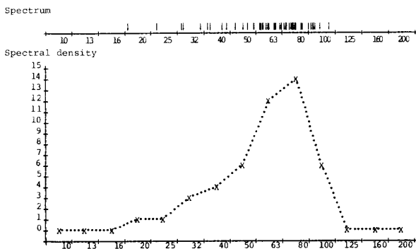
Fig. 8. Calculation of resonance modes.
