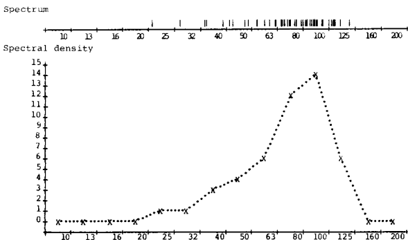
Fig. 7. Calculation of resonance modes.
