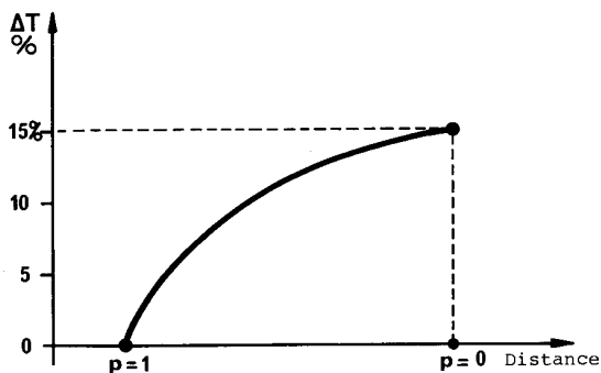
Fig. 16. Variation of RT of mode 2:1:0 (85 Hz), measured with a sinusoidal source, due to the movement of 4 m 2 of panels ( \alpha = 0.3 ), which represents 20% of the total inside area of the room.
