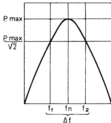
Fig. 2. Pressure versus frequency curve.
