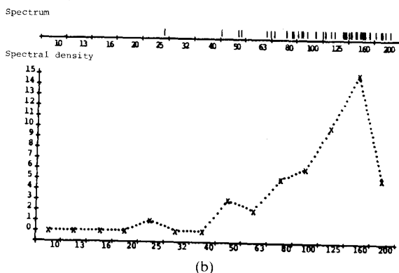
Fig. 12. Calculation of resonance modes: (a) 1.6:3:4; (b) 2:3:5.
