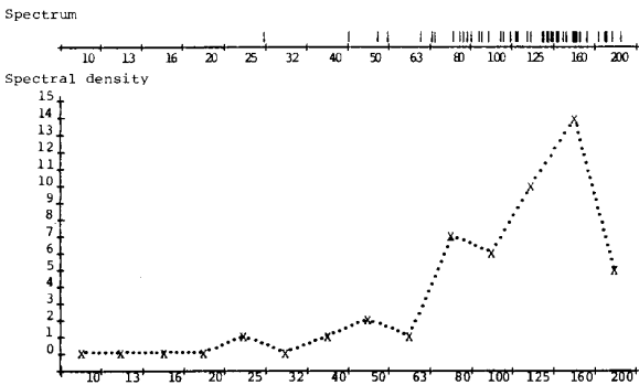
Fig. 5. Calculation of resonance modes.
