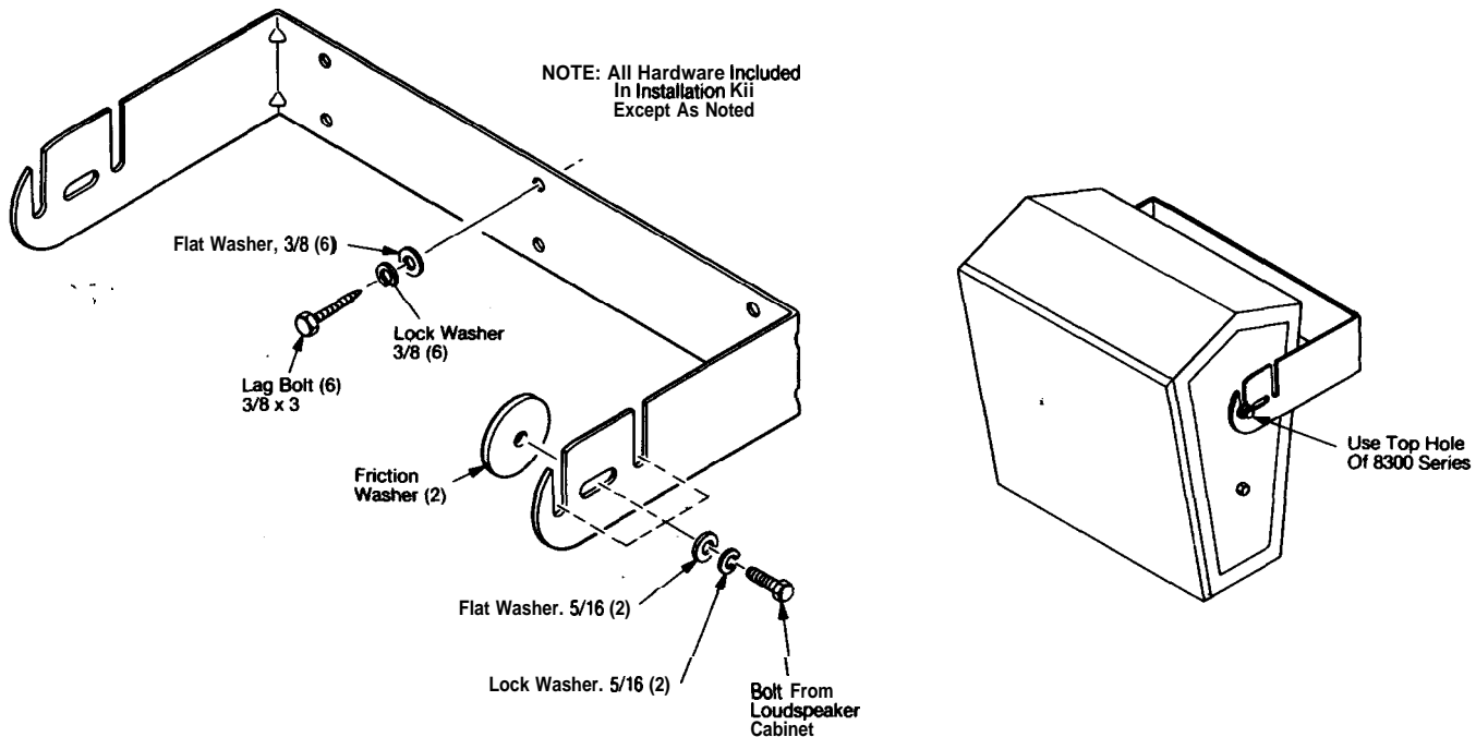
Figure 27. 2502 Wall Mount bracket used with 8300 series surround speakers
