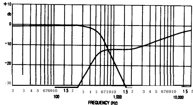
B. 500 Hz 16 dB/octave, with power response correction for 2360A Series horns
