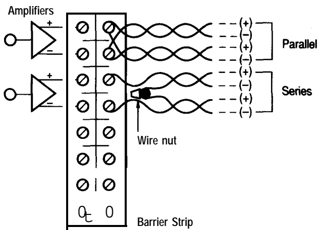
Figure 32B. Wiring at barrier strip in the booth
