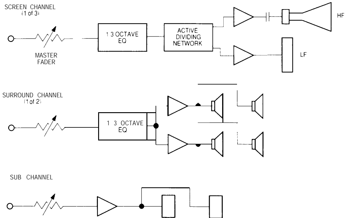
Figure 4C. Block diagram of B-chain with split surrounds
