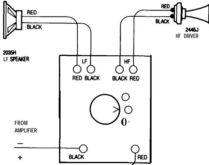
46738 wiring diagram
