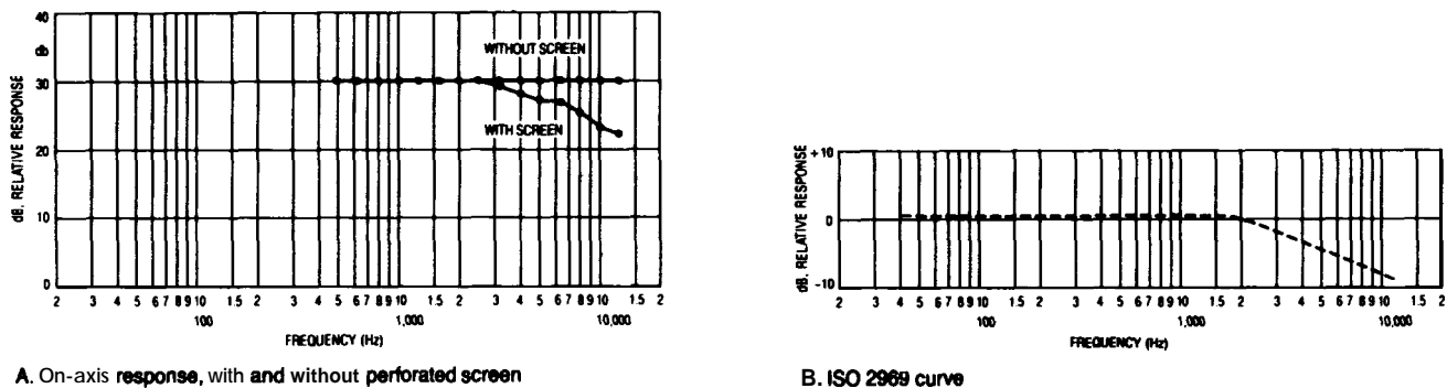
Figure 24. Screen losses and house equalization
