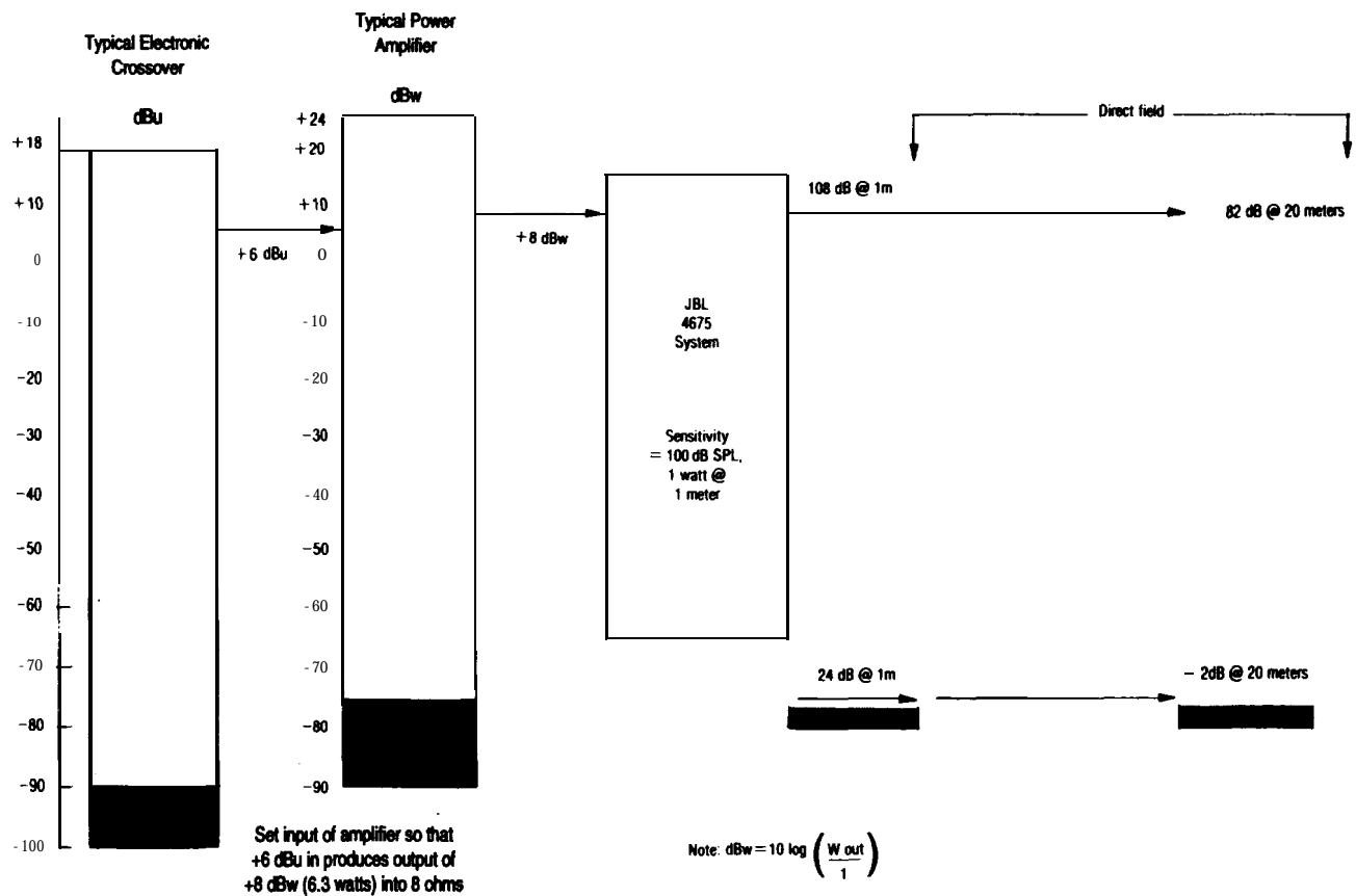
Figure 35. Typical gain-loss diagram for the B-chain of a cinema system
