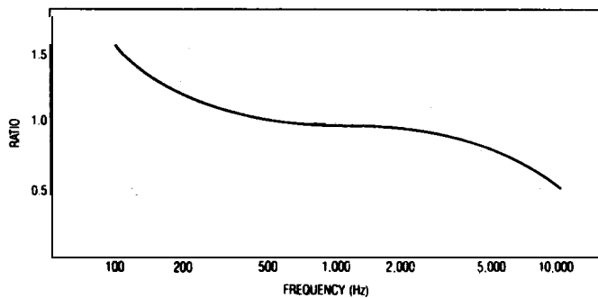
Figure 11. Variation of reverberation time with frequency
