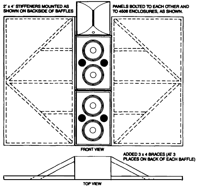
Figure 26. wings between screen loudspeakers.
