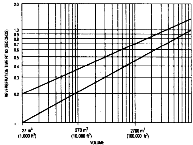
Figure 12. Suggested range of reverberation
