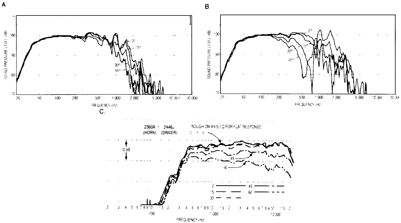
Figure 6. (A) Horizontal response; (B) Vertical response; (C) Off-axis response of a JBL 2360A horn equalized for flat power response
