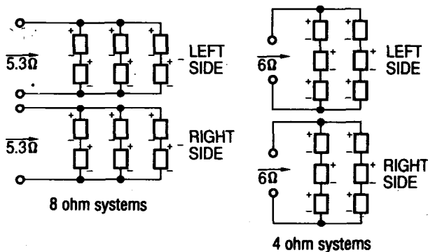
Figure 32A. Series-parallel hook-up
