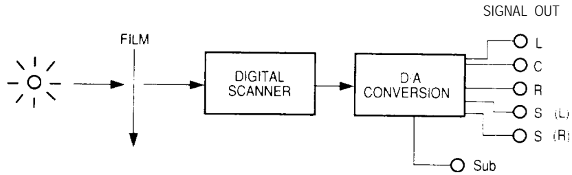
Figure 4B. Block diagram of digital A-chain
