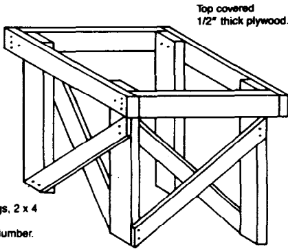
Figure 25. Isometric view of a platform .
