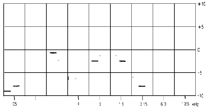
C. Reverberant (power) response of a cinema system composed of elements similar to those shown in Figures 5A and 5B
