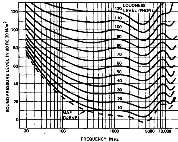
Figure 21. Robinson-Dadson equal loudness contours.
