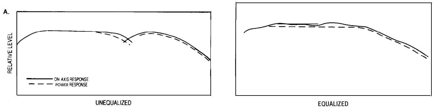
Figure 7. Cinema equalization of power flat systems
