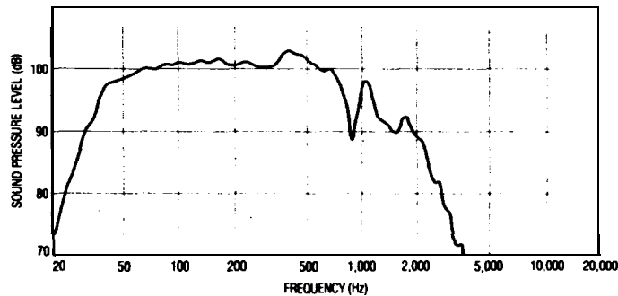
Figure 13. On-axis response of dual 360 mm (15 in.) 4636TH LF system.
