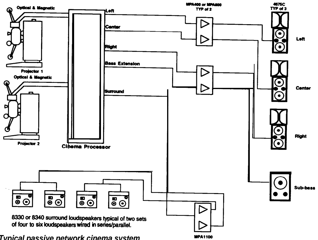
Figure 30. Typical passive network cinema system
