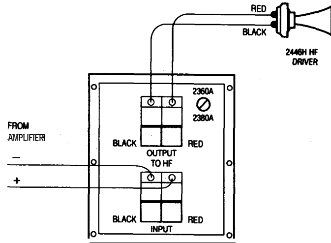
4675C wiring diagram
