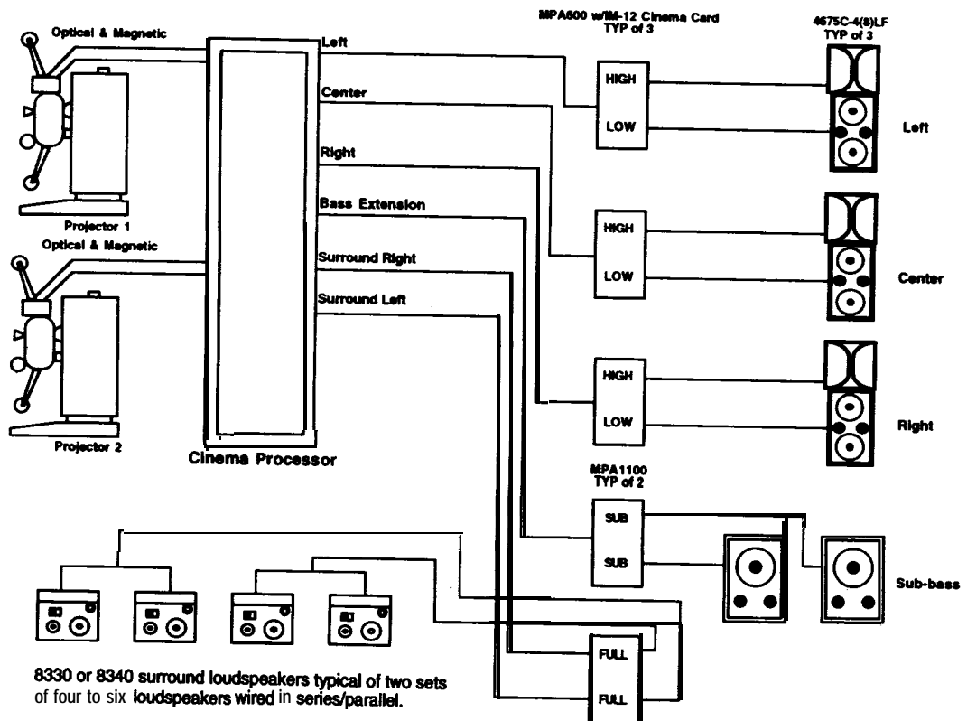
Figure 31. Typical biamplified cinema system
