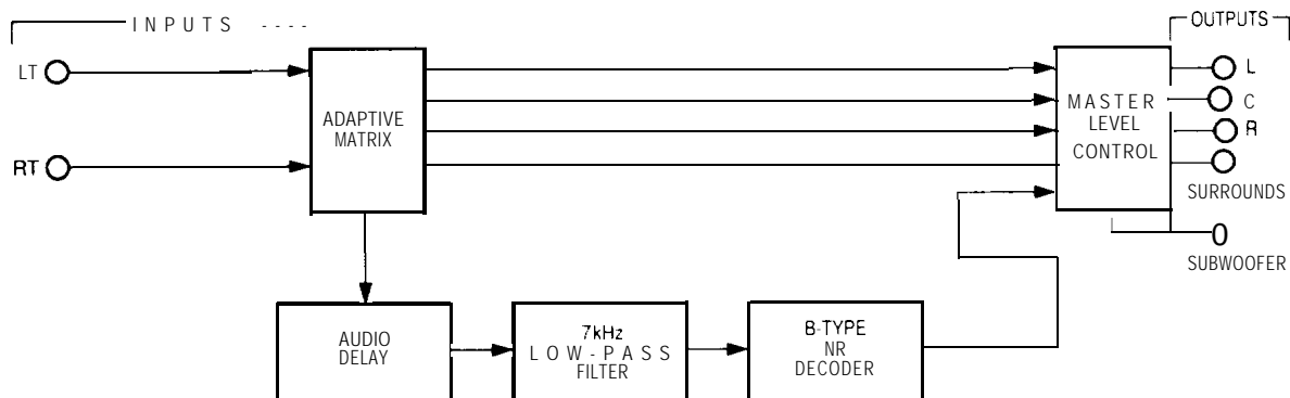
Figure 2B. Block diagram of the Dolby Stereo Optical playback matrix
