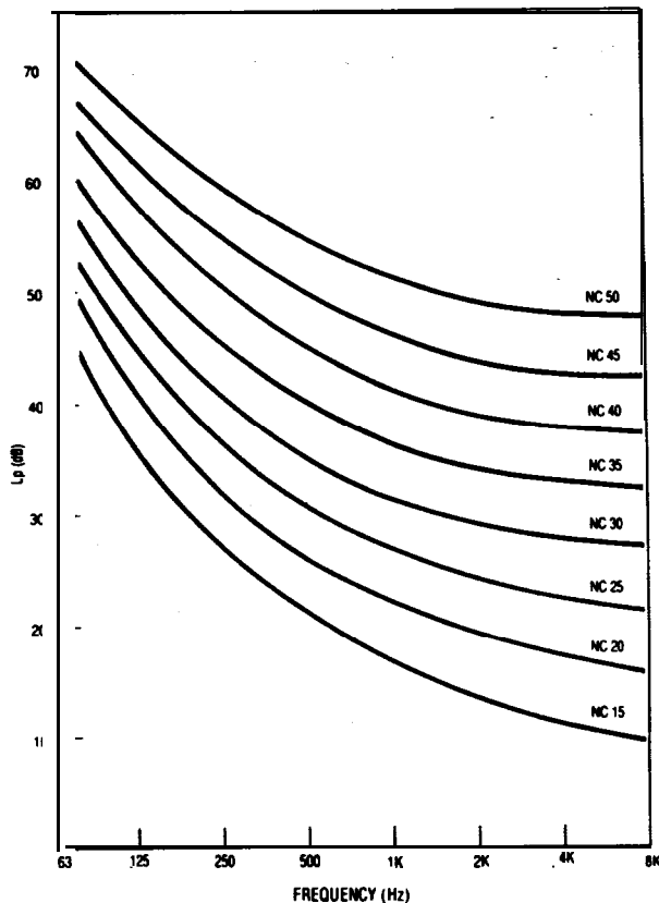
Figure 9. Noise Criterion (NC) curves, octave band data
