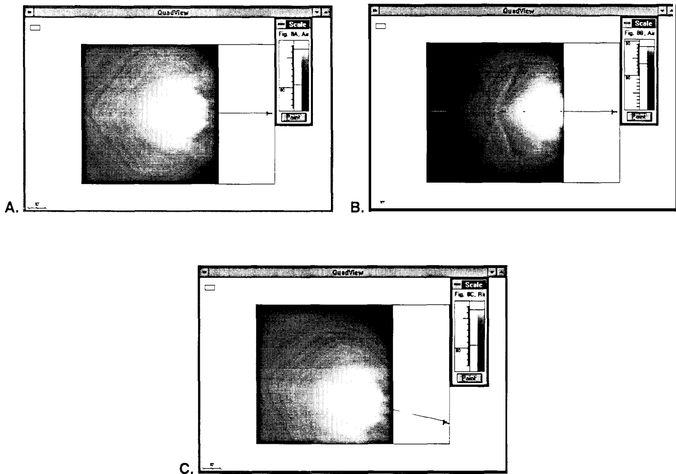
Figure 8. (A) Direct field coverage at 2kHz, aimed at rear wall; (B) Same, horn aimed 2/3 distance front to back; (C) Coverage of single outside horn.
