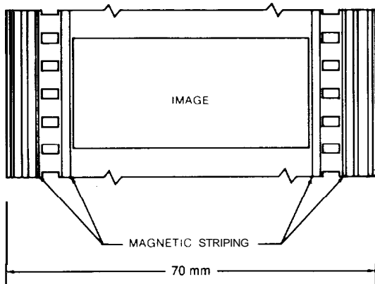
Figure 1. 70mm six-track magnetic format (A); 35mm four-track magnetic format (B)
