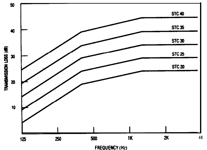
Figure 10. Sound Transmission Curves
