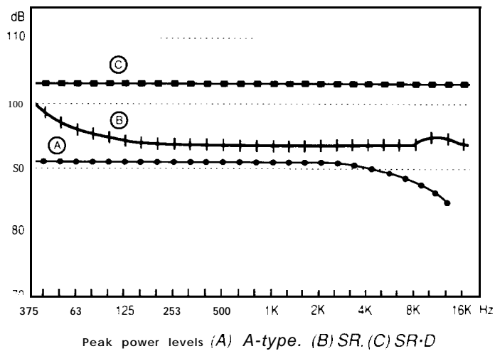
Figure 4D. Dynamic range requirements for Dolby-A, Dolby SR and Dolby SR-D formats
