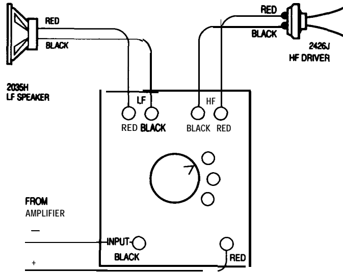
4671 B wiring diagram
