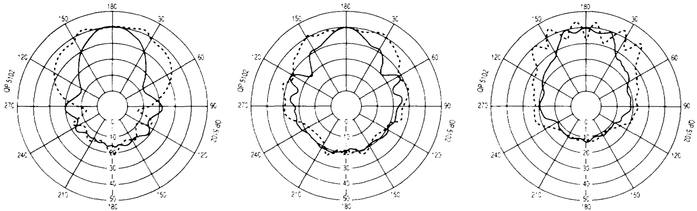
B. Polar characteristics of a 2 x 5 multicellular horn
