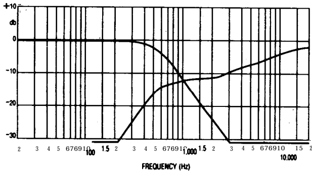
A. 500 Hz 12 dB/octave, with power response correction for 2360A Series horns
