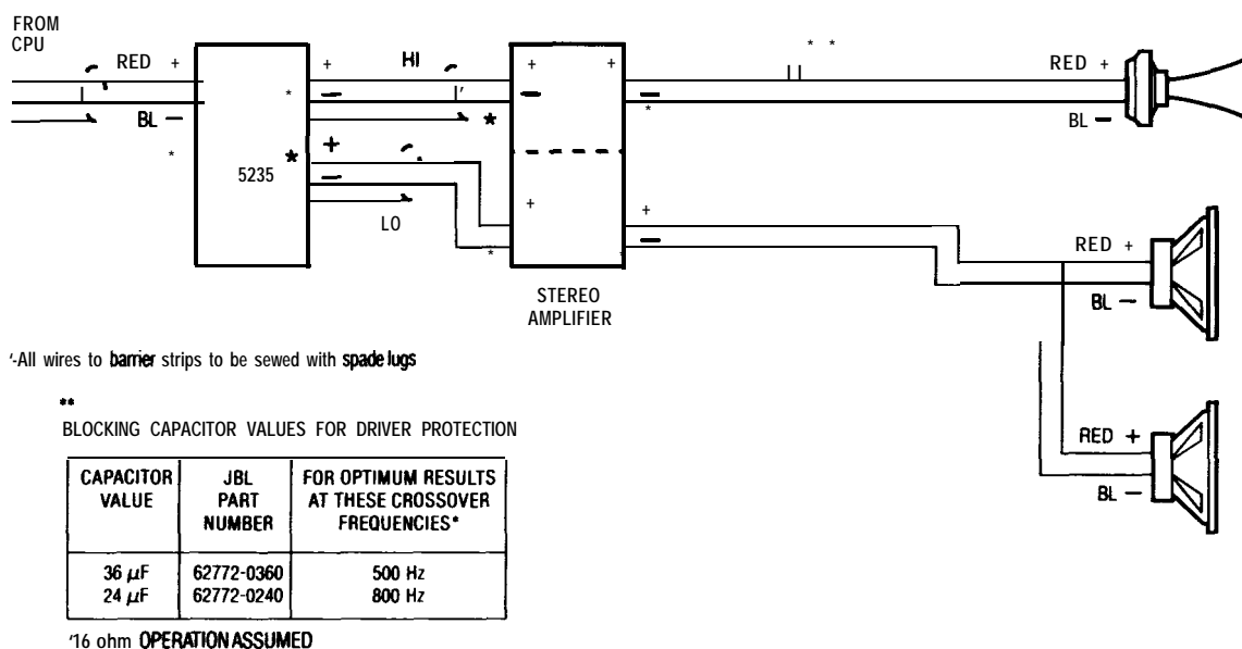
Figure 29. Wiring diagram for a bi-amp/i&d system
