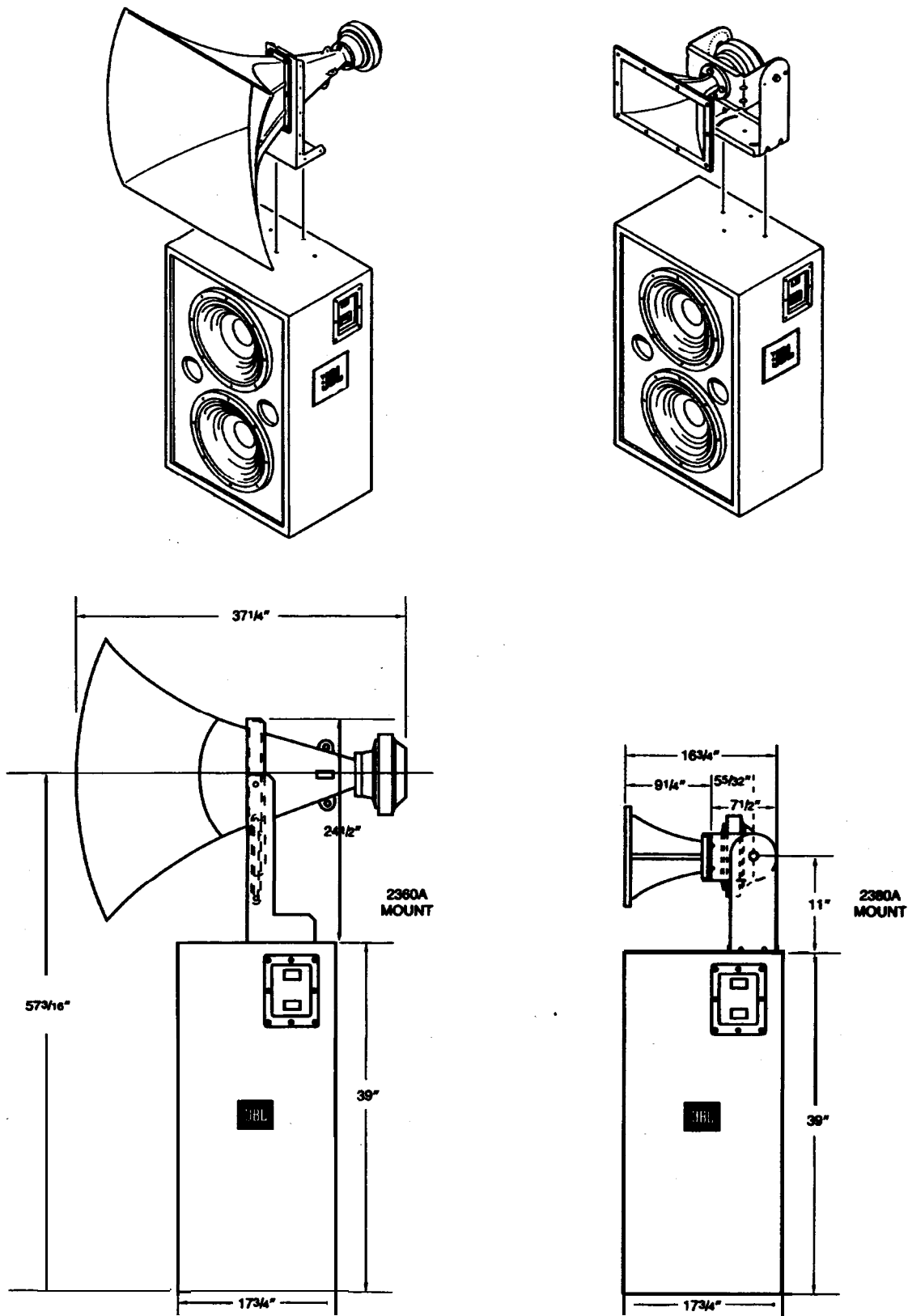
Figure 14. Complete system assembly diagram for 46700 and 46756.
