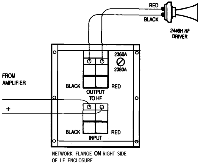
46700 wiring diagram
